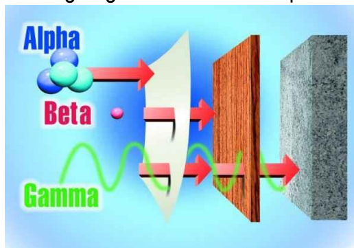
Fig.1 The interaction of radiation with matter
