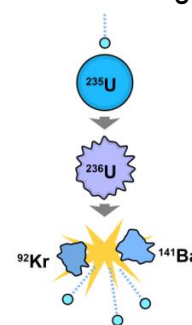
Fig.2 Nuclear fission
